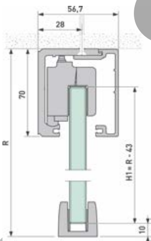
Montaje a techo Ceiling installation
