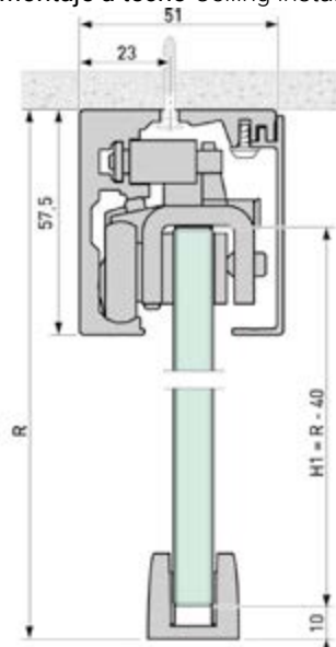
Montaje a techo Ceiling installation
